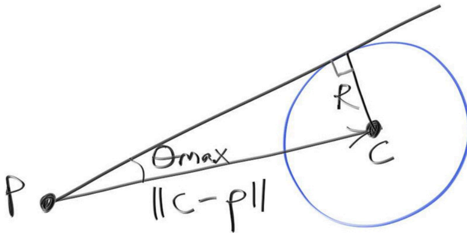
Figure 12: A sphere-enclosing cone
